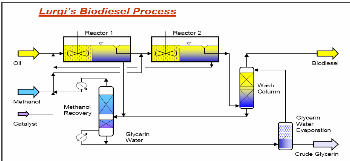
Fig. 12. Lurgi's biodiesel process (source: www.techbizindia.com/Article1 )
