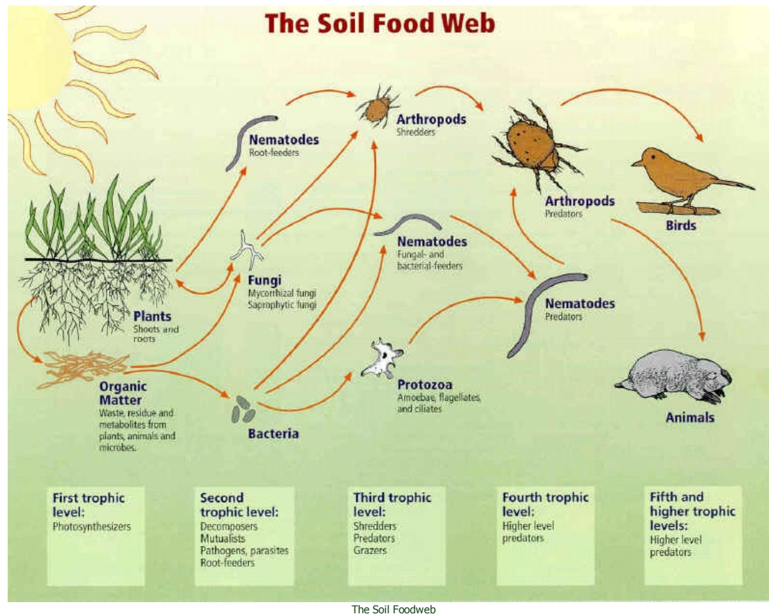
Figure 1: The Soil Food Web. From Ingham, E., et. al. 2000. Soil Biology Primer pg.5. Used with permission of Soil Foodweb, Inc. and Dr. Elaine Ingham.
