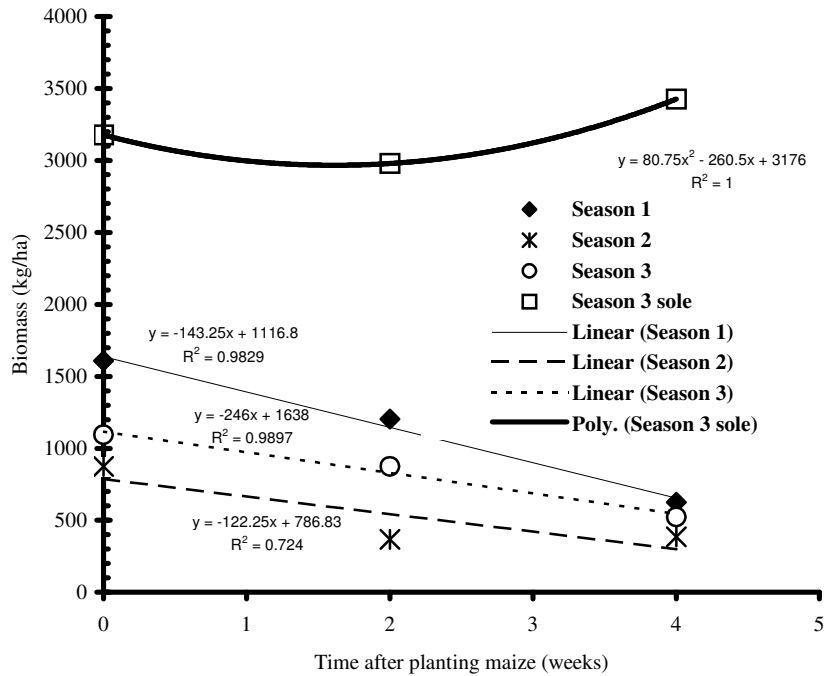
Figure 2. Effect of time of undersowing mucuna in maize on mucuna biomass
