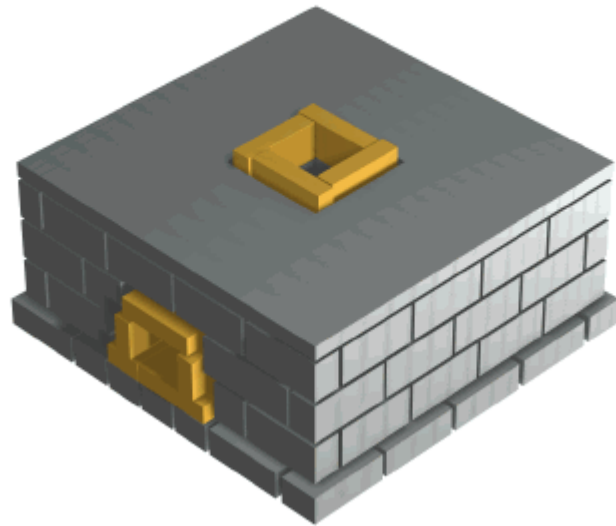
COMPLETED COMBUSTION CHAMBER
